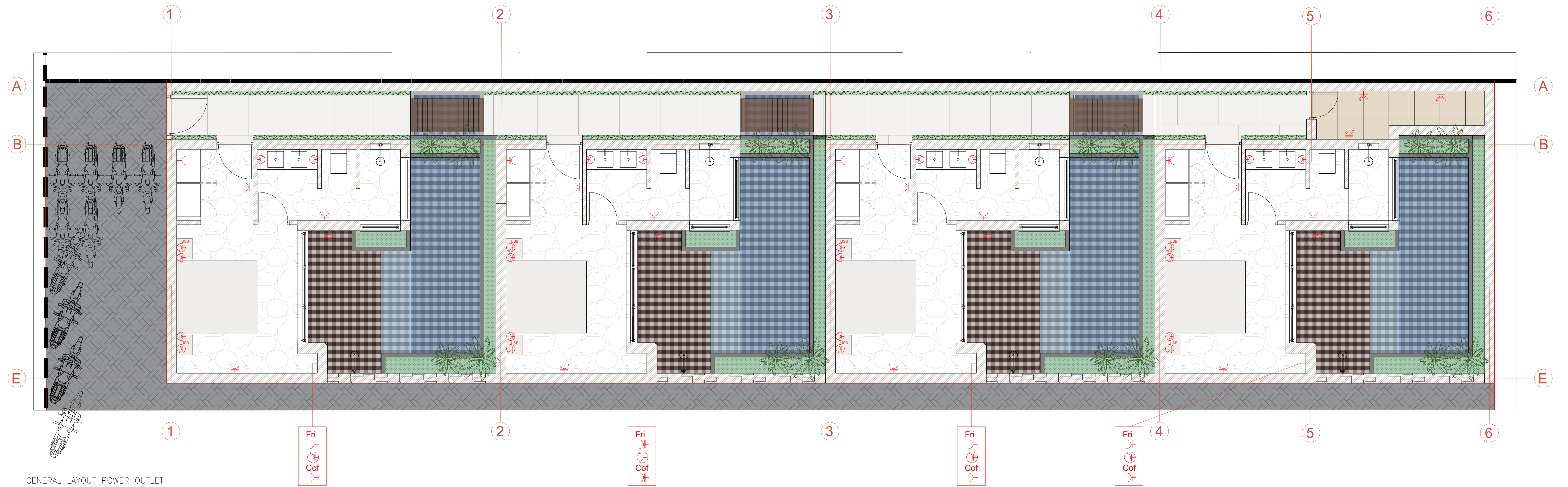
GENERAL LAYOUT POWER OUTLET
